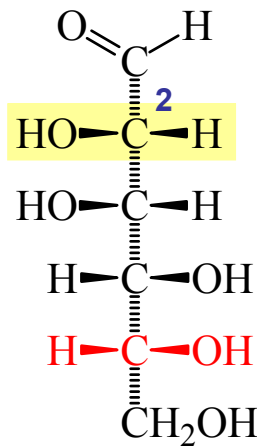
D(+)-mannosio
