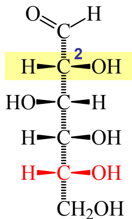
D(+)-glucosio
