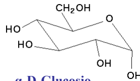
\alpha -D-Glucosio
